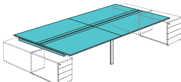
TP1M-01 2400x1620x740 TP1M-02 2800x1620x740 TP1M-03 3200x1620x740 TP1M-04 3600x1620x740
